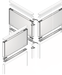
“T” connection
